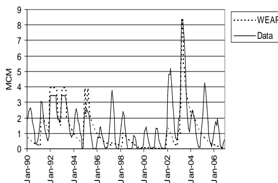
Figure 4 Kafrien Dam storage, historical data and WEAP estimate
