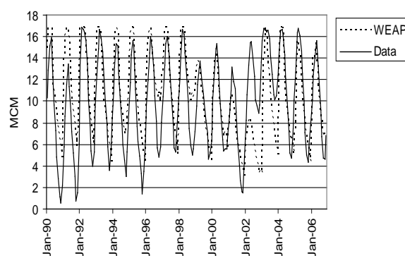
Figure 3 Wadi Arab Dam storage, historical data and WEAP estimate
