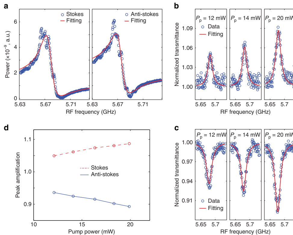
Figure 6 | Normalized transmittances of Stokes and anti-Stokes Brillouin signals and characteristic spectral Brillouin line shapes. (a) Spectrally resolved Stokes and anti-Stokes Brillouin lines shapes, respectively, obtained through heterodyne FWM experiments. (b,c) Normalized transmittances of Stokes and anti-Stokes Brillouin signals, respectively, for the m = 1 resonance of d = 0.8 \mu\text{m} BAM waveguide for the pump powers of 12, 14 and 20 mW. (d) Peak amplification (absorption) of Stokes (anti-Stokes) signals versus pump power obtained from the line shapes of b and c.
