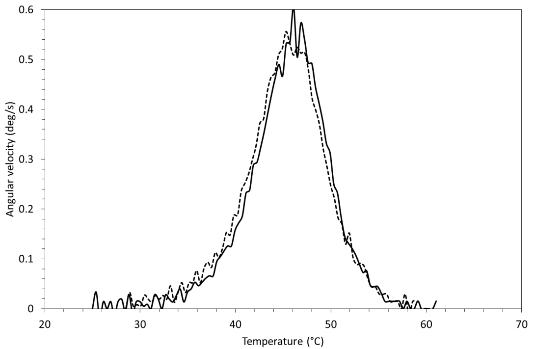
Fig. 7. Angular velocity during torsion recovery vs. temperature during stress-free heating at a constant temperature ramp of 0.9 °C/min for two shape memory epoxy samples.
