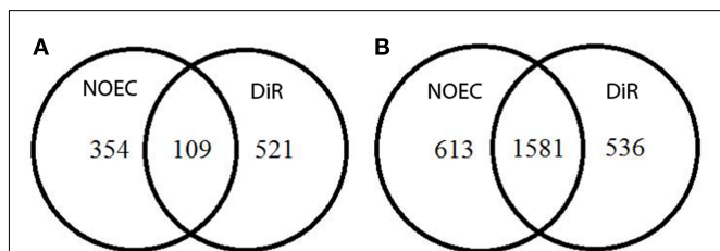
FIGURE 3 | Venn diagrams showing the number of genes responding to NOEC and DiR levels of toxicants in the Soil exposure (A) and in Extract exposure (B).
