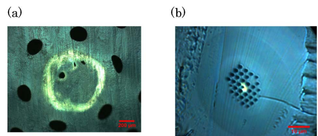
Fig. 2. In both images, the bright part is the doped region. (a) Doped cane. (b) Doped fiber.
