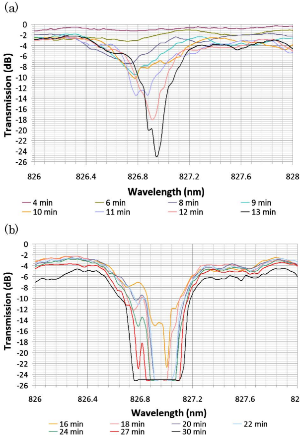
Fig. 3. Growth spectrum FBG. (a) First 13 min of inscription. (b) Inscription from 16 to 30 min.
