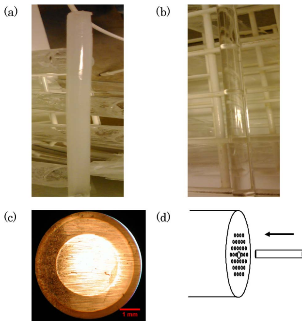
Fig. 1. Doped rod (a) 10 s and (b) 10 min after extraction from the solution. (c) Transverse structure of doped rod. (d) Microstructured preform with a larger central hole for the doped rod.
