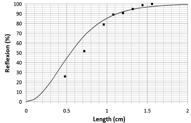
Fig. 4. Reflection against grating length. The solid line is the theory and dots the experimental results.
