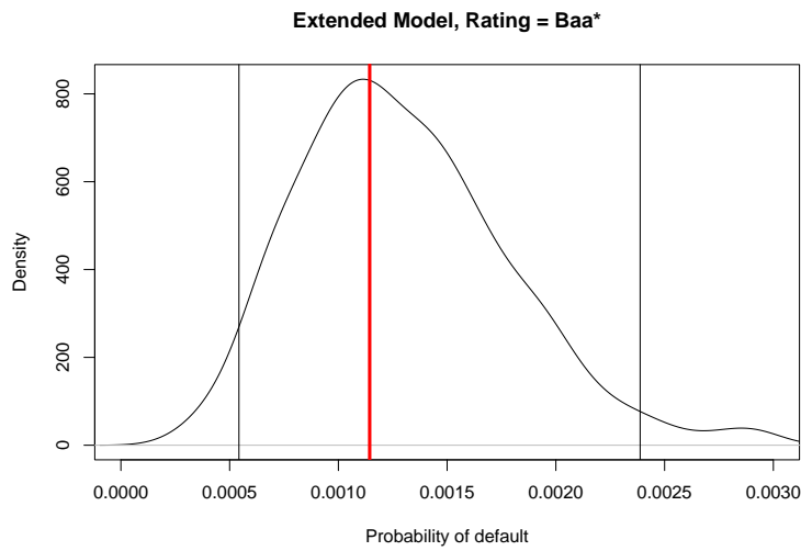
Figure 3: Simulated density distribution of the default probability estimates for Baa (the top graph) and Baa* in the extended model over the period 1987-1991. The bold vertical lines show the one-year default probability (PD) corresponding to the 'true' value derived from the estimated transition probability matrix. The thin vertical lines mark the 2.5% and the 97.5% quantile.
