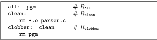
Figure 3: Building from scratch is often invoked upon cleaning up with targets such as clobber . If added to the rules of Figure 1, R_{\text{clean}} deletes intermediary files, and R_{\text{clobber}} deletes all files.
