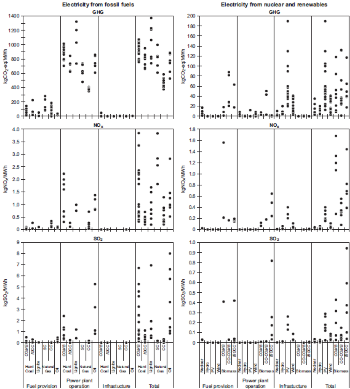
Figure 1. Life cycle emission factors for electricity generation from selected technologies, divided into “fuel provision”, “plant operation” and “infrastructure”, according to the LCA studies reviewed
