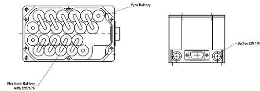
Figure 63. Battery Pack
