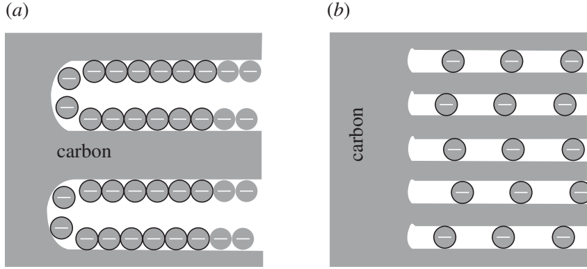
Figure 4. Electrochemical double-layer charge (a) according to the Helmholtz model and (b) in sub-nanometre pores.
