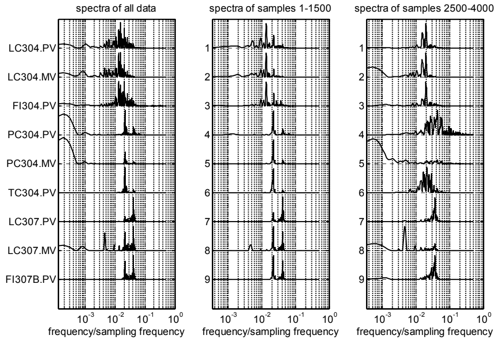
Figure 5. Spectra from the data set and sub-sets
