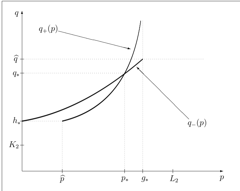
Figure 7. A computer drawing of the functions q_+(p) and q_-(p) .
