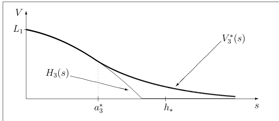
Figure 3. A computer drawing of the payoff function H_3(s) and the value function V_3^*(s) , when (1.2.10) holds for L_1 and L_2 .
