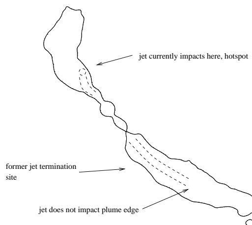
Fig. 7. Schematic of the possible current situation in 3C 130.
