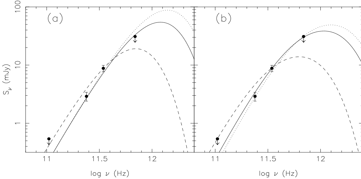
Figure 4. Comparison of the mm/submm spectrum of CUDSS14A with that of (a) M82 and (b) Arp220 at z=2.0 (dots), 2.5 (solid) and 5 (dashed) with arbitrary shifts in absolute flux level. Note that the M82 spectrum is not consistent with the data for z=2.0 but is just consistent for z=5 , whereas Arp220 is just consistent at z=2.0 but is not consistent for z=5 . Thus for these templates we can constrain the redshift to the range 2.0 to 5.0.
