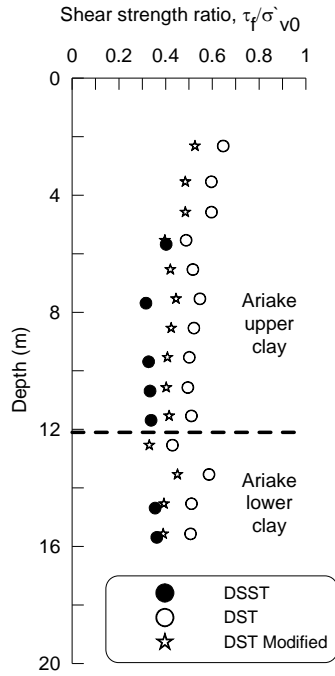
Fig. 9. Shear strength ratios from DSST, DST and DST modified to take into account strain rate and shearing mechanism effects for Ariake clay
