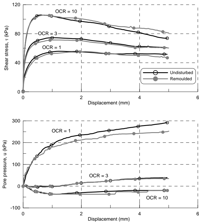
Fig. 13. Comparison of DST tests on remoulded and undisturbed specimens of plastic Drammen clay.
