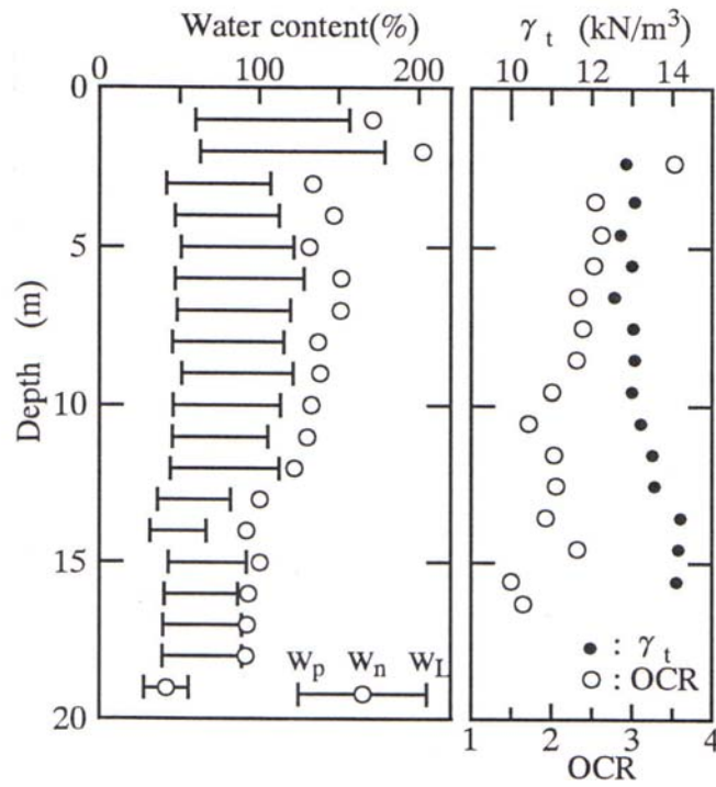
Fig. 4. Basic physical properties and degree of overconsolidation of Ariake clay (Tang et al., 1994)
