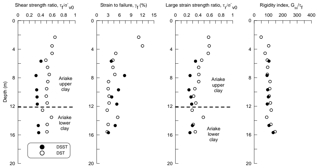
Fig. 6. Shear strength and stiffness data for DSST and DST tests in Ariake clay
