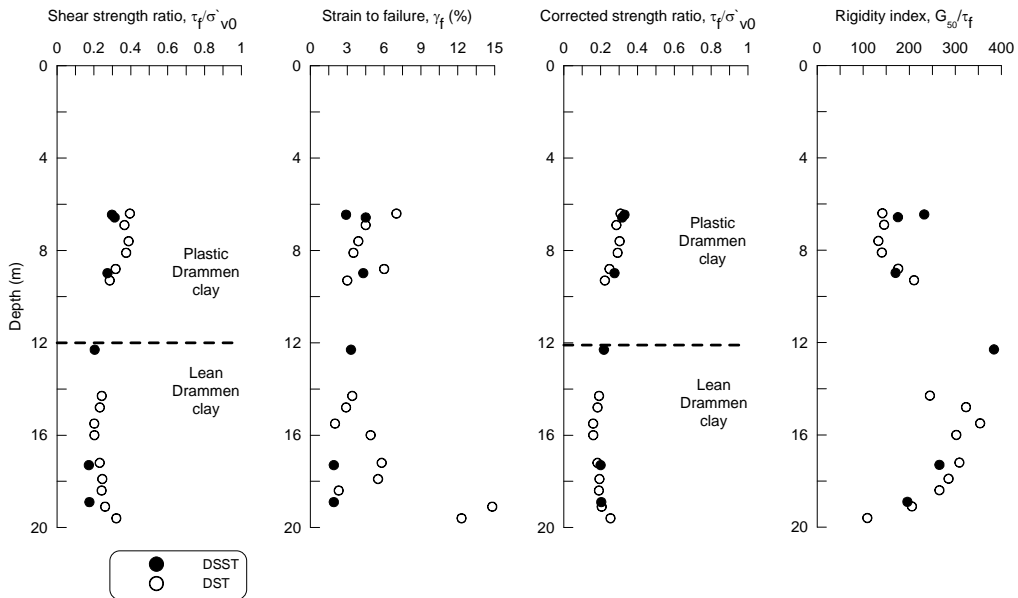
Fig. 10. Shear strength and stiffness data for DSST and DST tests in Drammen clay
