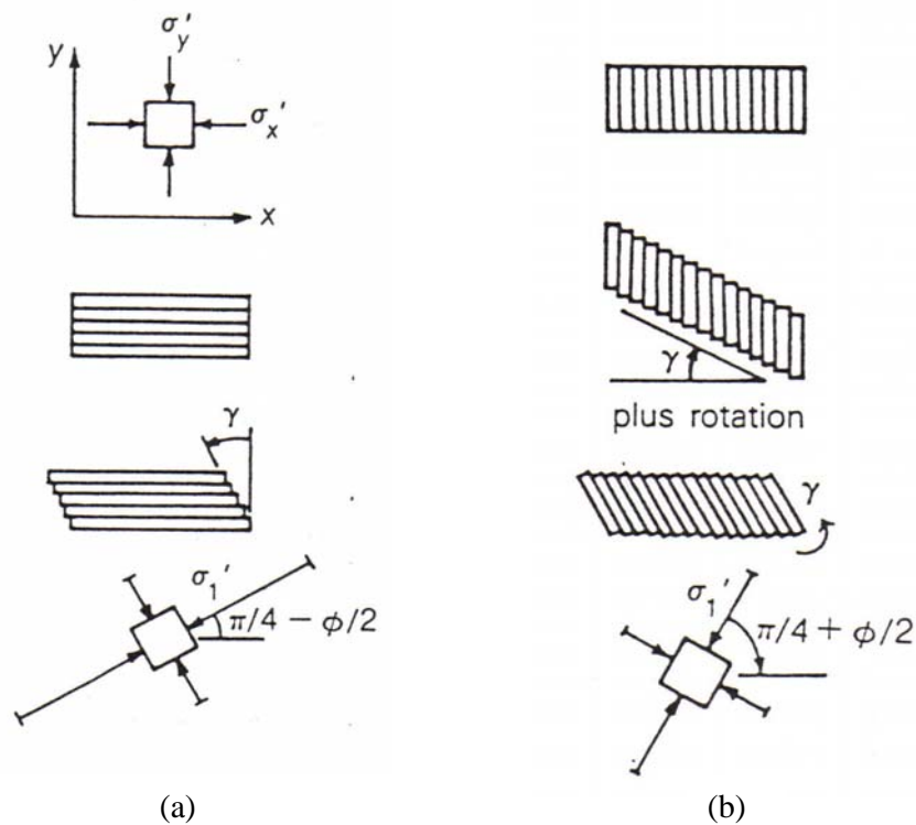
Fig. 2. Two possible mechanisms which can occur during shear; (a) one of translation along a series of horizontal planes, or (b) one of translation along vertical planes with an associated rotation of those planes (Josselin de Jong, 1972 and Wroth, 1984)
