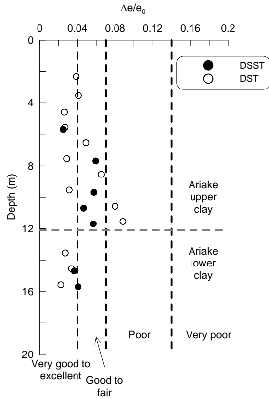
Fig. 7. Assessment of sample quality for Ariake clay using NGI criteria of Lunne et al. (1997)
