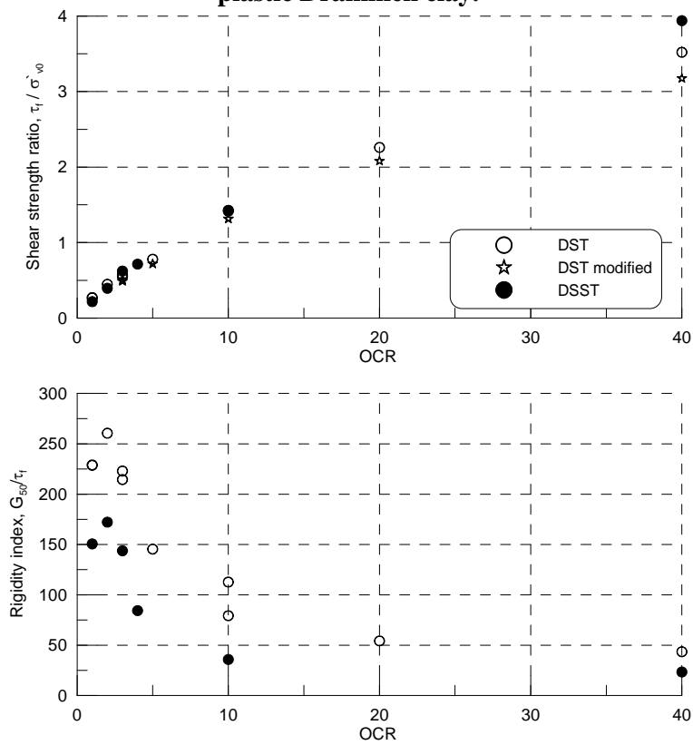
Fig. 14. Comparison of shear strength ratio at failure and rigidity index for overconsolidated specimens of plastic Drammen clay.
