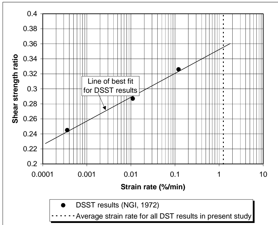
Fig. 12. Effect of strain rate on the DSST shear strength ratio of Drammen clay (NGI, 1972).
