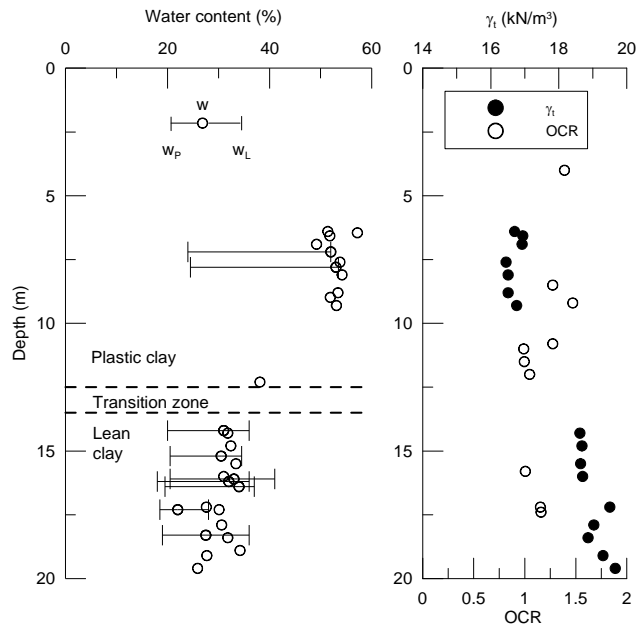
Fig. 5. Soil profile at Drammen Museum Park / Danvikgata site (Lunne et al., 1976, Lunne and Lacasse, 1999)
