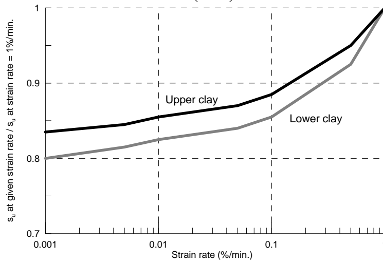
Fig. 8. Influence of strain rate for K_0 consolidated triaxial tests on Ariake clay (Hanzawa et al., 1990)
