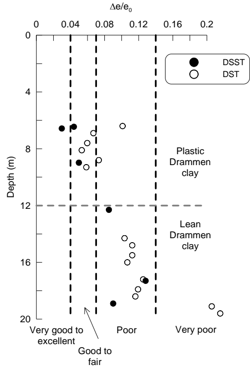
Fig. 11. Assessment of sample quality for Drammen clay using NGI criteria of Lunne et al. (1997)
