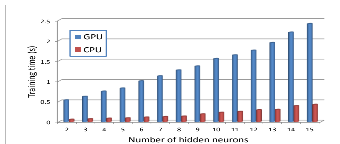
Fig. 4. Relative times taken to train a single ANN using the ultrasonic data with different numbers of hidden neurons.
