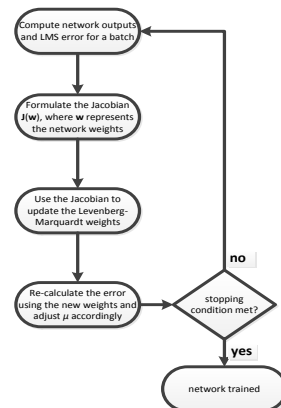
Fig. 2. Flow diagram outlining the procedure for using the Levenberg- Marquardt training algorithm
