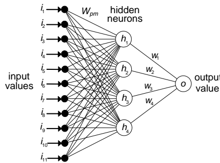
Fig. 1. Example of an MLP ANN with a single output
