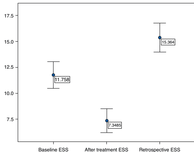
Figure 1 Epworth score.
