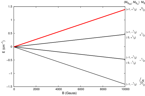
Fig. 2. (color online). \text{Li}(^2S) + \text{NH}(X^3\Sigma^-) thresholds as a function of magnetic field. The spin-stretched ( m_{s\text{NH}} = +1, m_{s\text{Li}} = +\frac{1}{2} ) M_S = +\frac{3}{2} state is shown in red.
