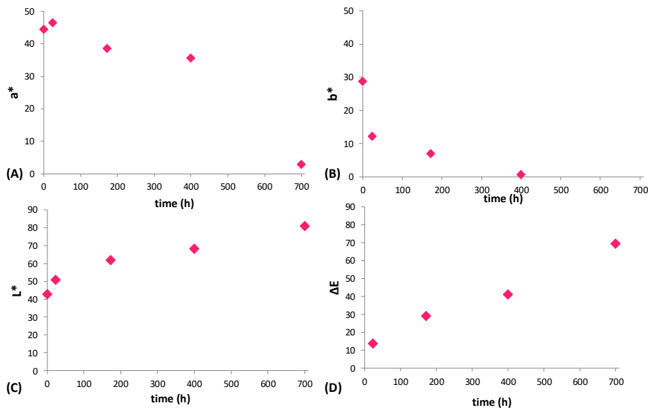
Figure 2: Results of the colorimetric analysis of the paint replica subjected to increasing doses of UV-Vis light (accelerated ageing) in CIELAB coordinates: values of a* (A); b* (B); L* (C) and ΔE (D) with ageing time.
