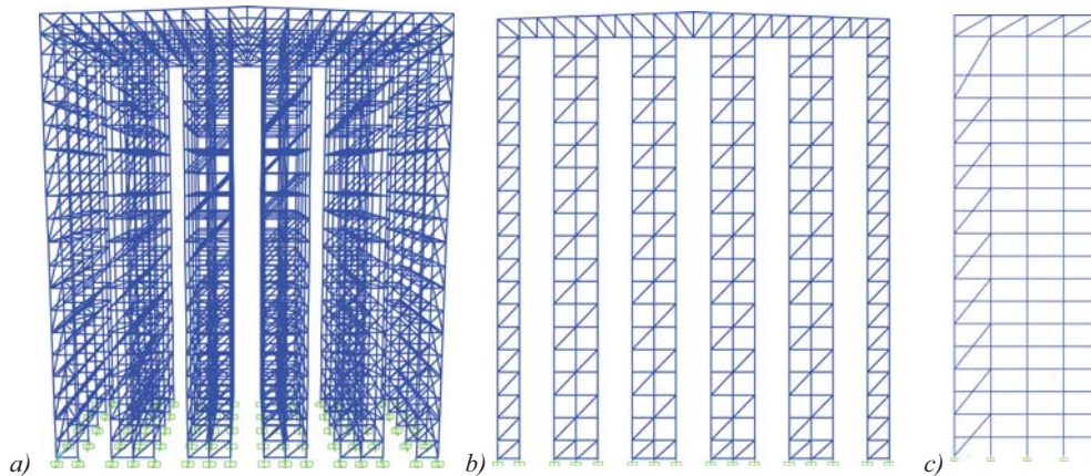
Fig. (3). Three-dimensional model for the designed ARSW building: a) global view; b) transversal view; c) longitudinal view.
