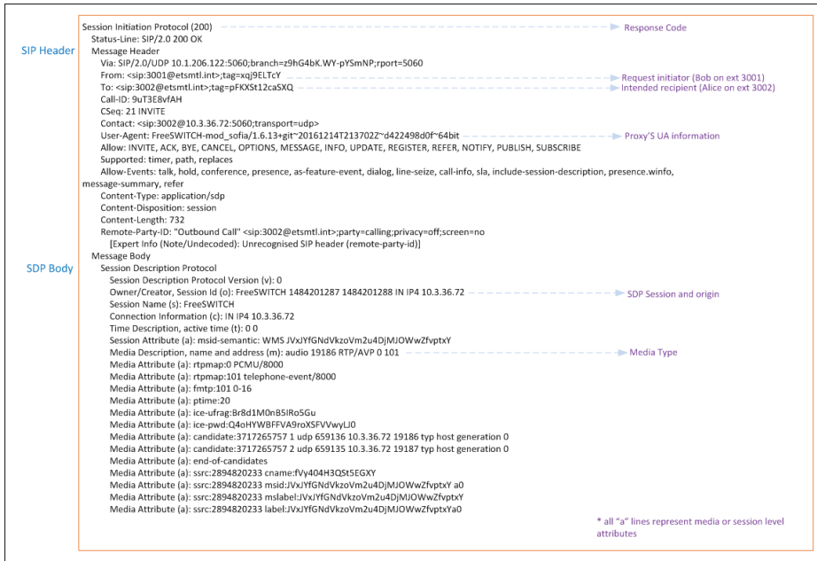
Figure 2.19 SIP OK (Proxy to Bob).
