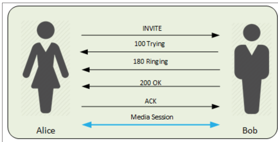
Figure 2.4 Three-way handshake.
