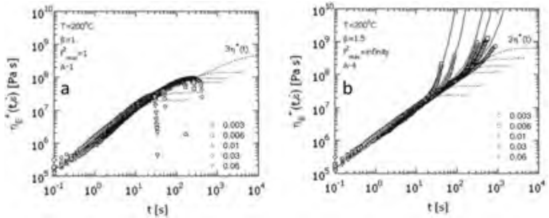
FIG. 1.15 Tensile stress growth coefficients of a (a) linear PMMA, (b) cross-linked PMMA. The viscoelastic limit is indicated by 3\eta^+ , the other dotted lines and plain lines are the predictions of various models not described here. Extracted from [71]
