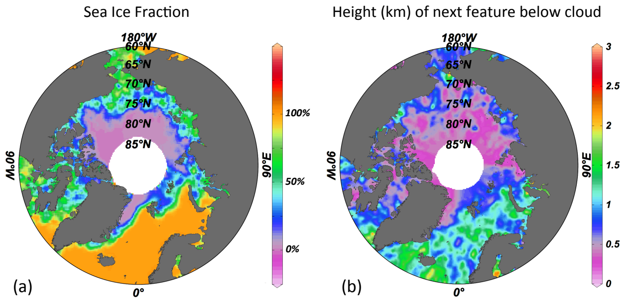
5 Figure 3: The weighted-average gridded maps of features below individual cloud points from Fig. 1b for a) sea ice fraction, and b) height of the next lowest feature associated with individual cloud profiles, where a value of 0 indicates that the ocean surface or sea ice was the next lowest feature. Over open ocean, ONLi clouds were much more likely to overlay another cloud than over sea ice.
