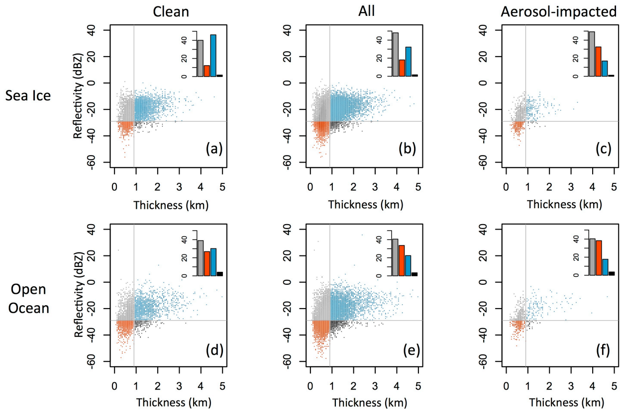
5 Figure 4: A comparison of CALIPSO ONLi cloud thickness (km) with CloudSat reflectivity (dBZ), as separated by sea ice and open ocean regimes, and by clouds found in conditions labelled as clean background, all conditions, and aerosol-impacted conditions. To better show changes in the two parameters, plots have been divided into four quadrants (above (grey and blue) and below (orange and black) the CloudSat reflectivity detection limit of -29 dBZ), and above (blue and black) and below (orange and grey) a thickness of 0.9 km. In the upper right of each plot is shown the percent of cases within each quadrant, following the quadrant color scheme. Points represent clouds > 750 m asl.
