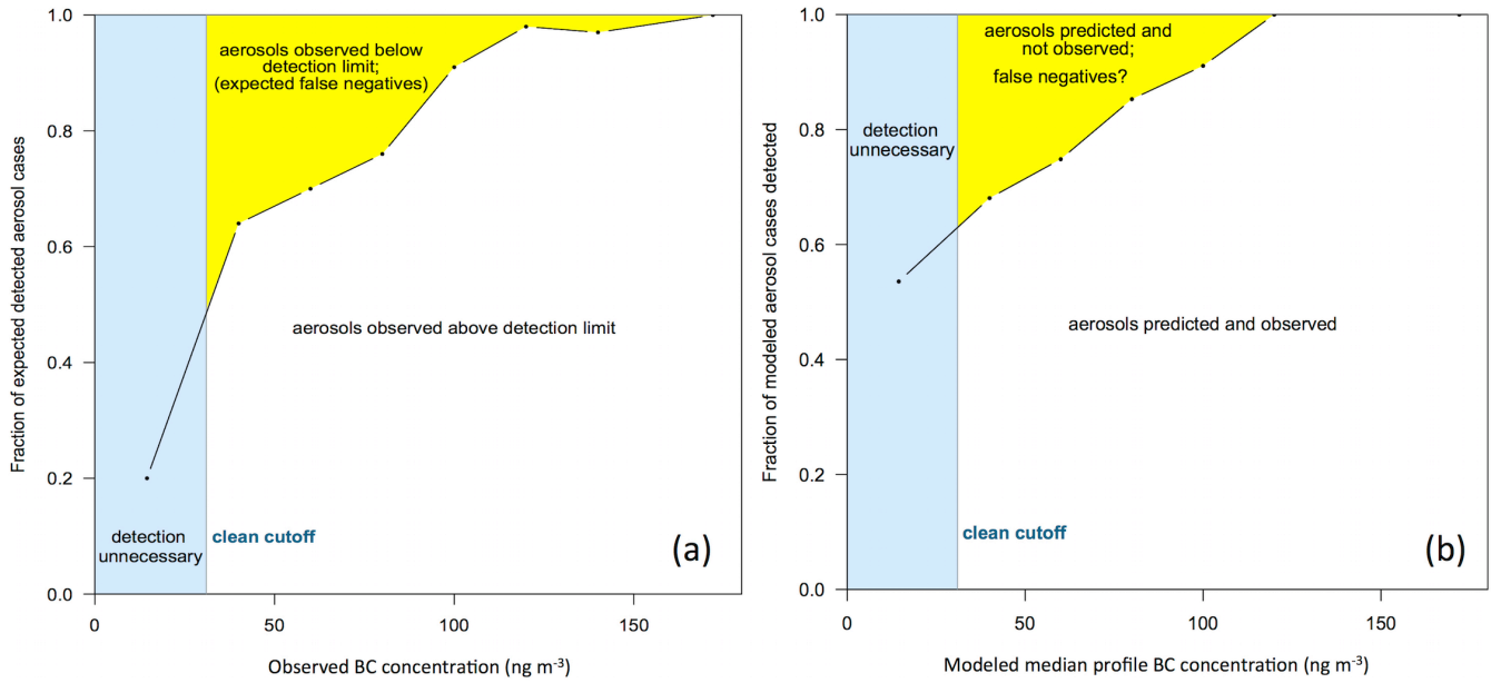
5 Figure 2: Based on CALIPSO Arctic profiles under non-cloudy conditions, we compare a) the expected fraction and b) possible maximum fraction of false negatives (aerosol present but not detected) for the combustion tracer, black carbon (BC, \text{ng C m}^{-3} ). The expected fraction of false negatives in panel a) was determined by comparing binned out-of-cloud 2008 ARCTAS-A and -B BC concentrations with the fraction of the total number of samples between 1-5 km that had converted backscatter values ( \text{Mm}^{-1} \text{sr}^{-1} ) above the CALIPSO clear-sky nighttime backscatter detection limit from Winker et al. (2009) (see text for more details). Possible maximum false negative values in panel b) were determined by comparing the FLEXPART model's median BC concentrations between 0-10 km with the fraction of the total CALIPSO profiles under non-cloudy conditions during January, 2008 where aerosols were not detected. The clean cut-off below 10 which air is taken as "clean" is assumed to be 30 \text{ ng BC m}^{-3} .
