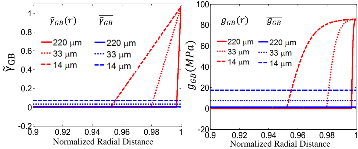
Figure 4 (a) \tilde{\gamma}_{GB} profile and the effective \overline{\tilde{\gamma}_{GB}} (horizontal lines) (b) g_{GB} profile and the effective \overline{g_{GB}} (horizontal lines)
