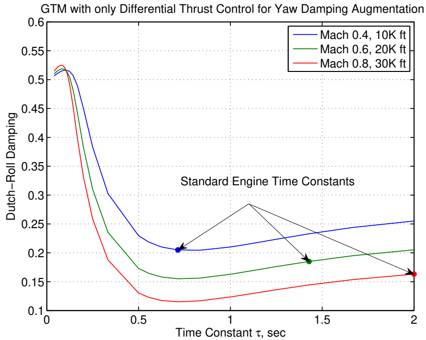
Figure 49: Dutch-Roll Damping of GTM Using Differential Thrust Control without Rudder
