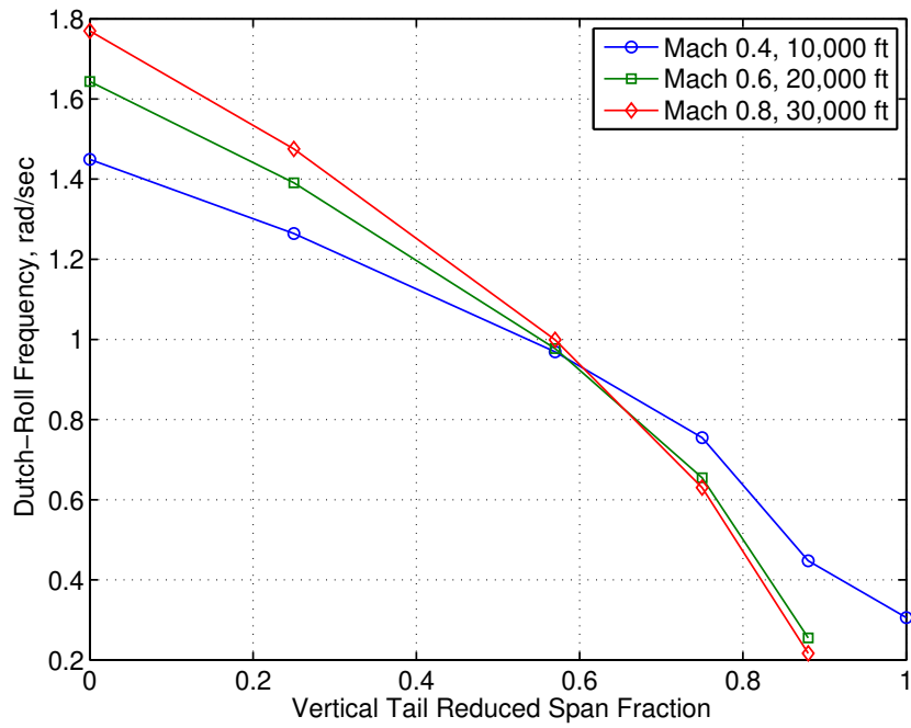
Figure 42: Frequency of Dutch-Roll Mode of the GTM as a Function of Vertical Tail Reduced Span Fraction
