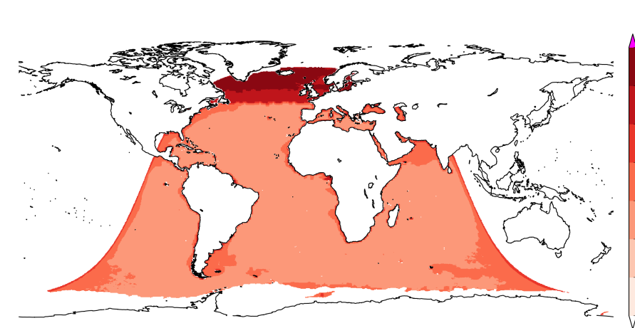
Figure 3: Monthly mean of the ratio of shortwave radiation absorbed within the diurnal warm layer to the net surface shortwave radiation for 12UTC, Dec 2017.
