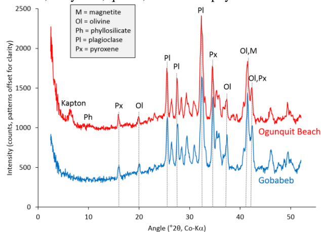
Fig. 2. CheMin XRD patterns of OG and GB, with major peaks labeled. Note: OG was analyzed in a cell with Kapton windows, producing an artifactual peak at ~6 °2θ.
