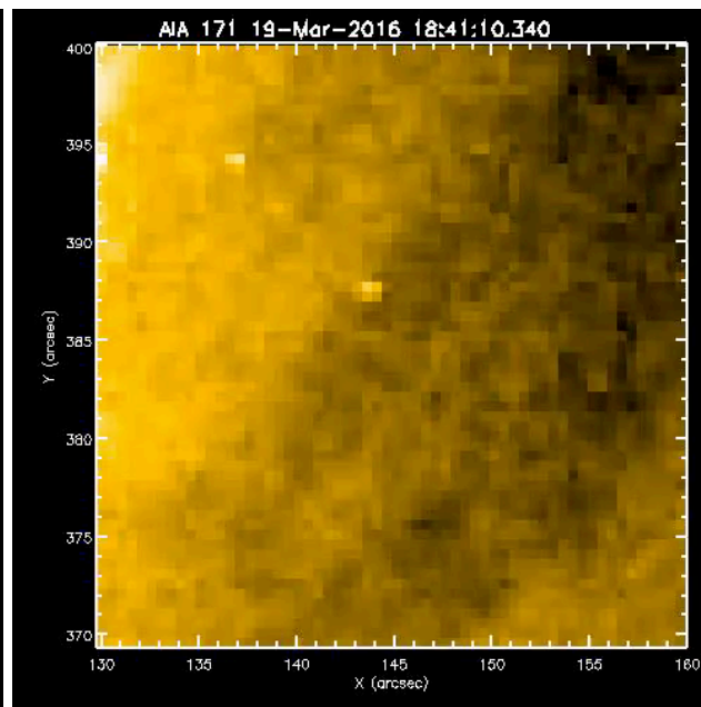
AIA 171
