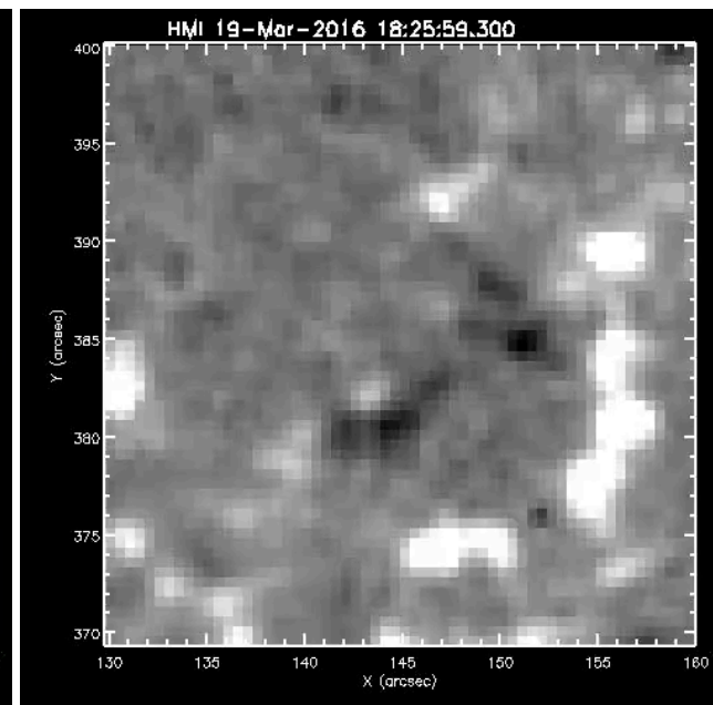
HMI
