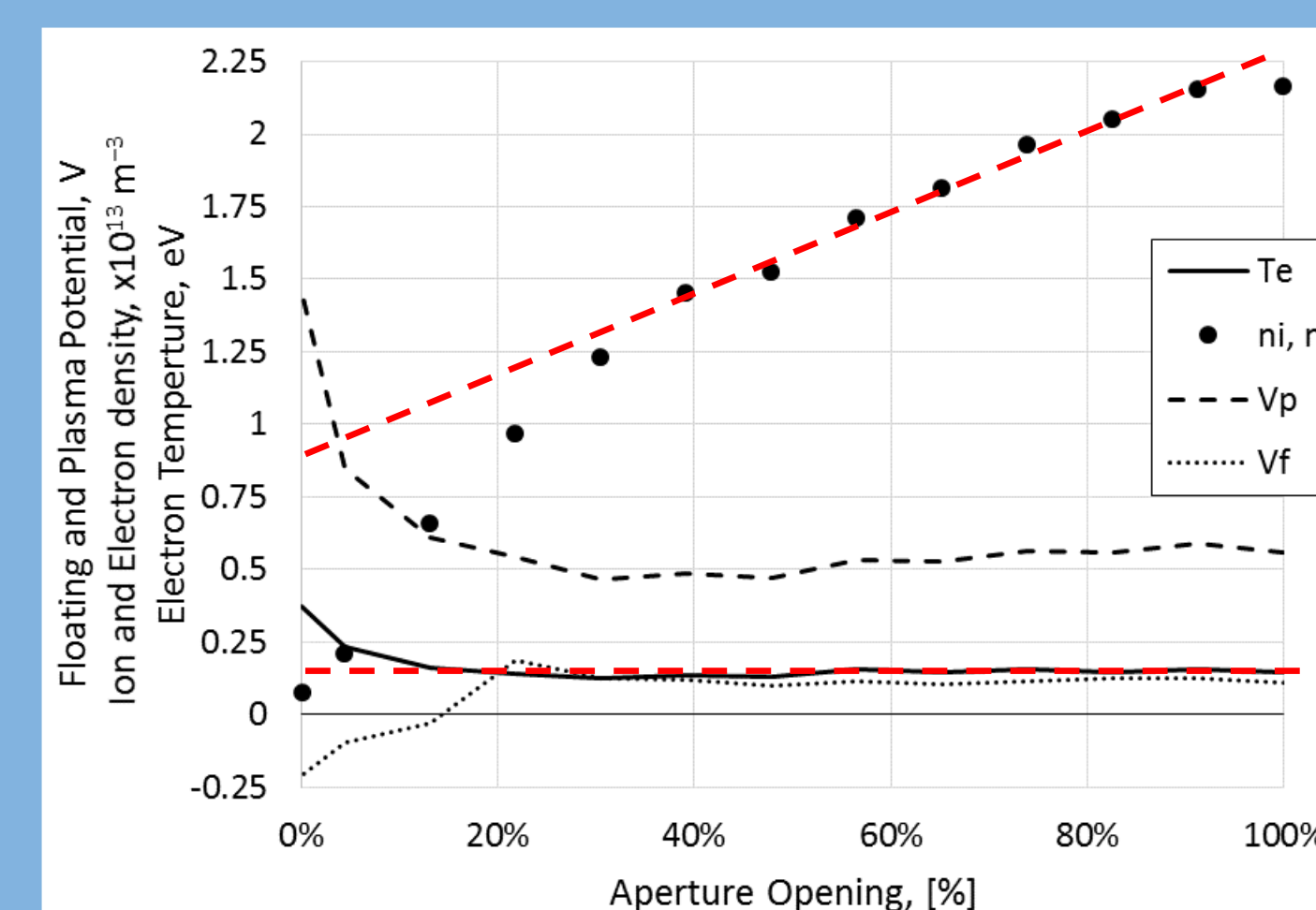
The response of the electron and ion densities can be characterized
