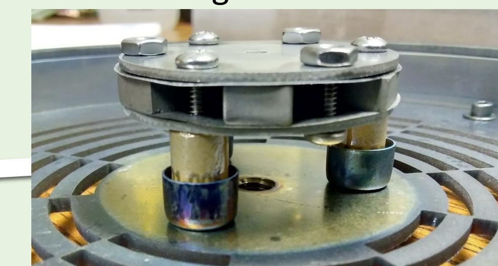
High energy electrons are prevented from exiting the source via a ring cusp magnetic filter. We increased the number of magnets to increase the filtering capability (i.e., decrease the electron temperature). This becomes increasingly more important when the source become hot through Joule heating.
