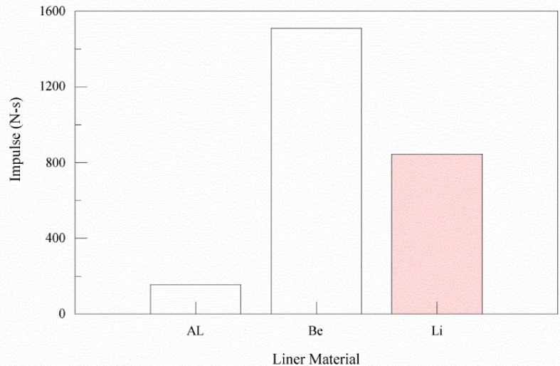
Fig. 16 Impulse as a function of target liner material
