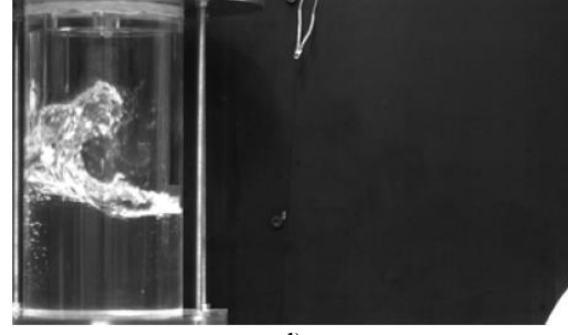
Figure 37. Comparison of interface motion and temperature field at the center plane of the tank between current k-\omega SST (a) and LES (b) models; results of simulation of Himeno et al. [2] (c) and the experiment (d) after 1.0 seconds of sloshing
