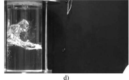
Figure 26. Comparison of interface motion and temperature field at the center plane of the tank between simulations w/o tank wall (a), with the tank wall (b) and Himeno et al. [2] (c) and experiment (d) after 1.0 seconds of sloshing
