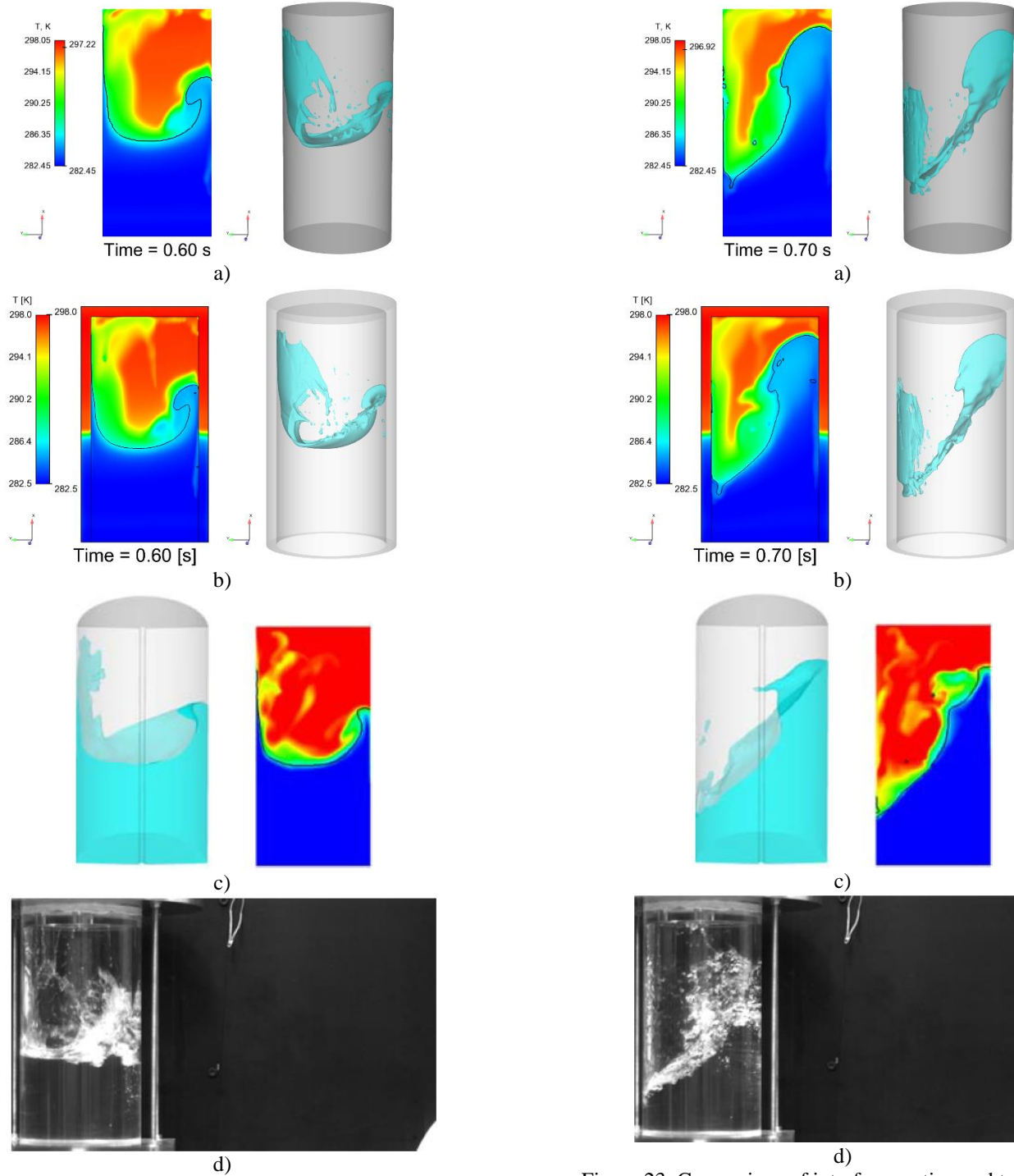
Figure 22. Comparison of interface motion and temperature field at the center plane of the tank between simulations w/o tank wall (a), with the tank wall (b) and Himeno et al. [2] (c) and experiment (d) after 0.6 seconds of sloshing
