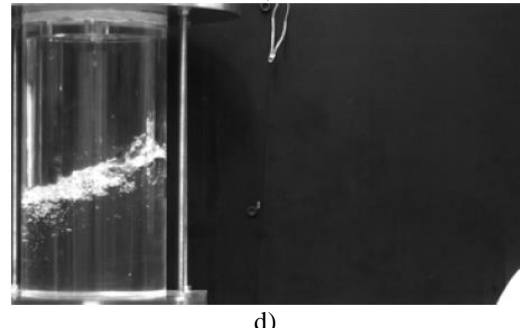
Figure 27. Comparison of interface motion and temperature field at the center plane of the tank between simulations w/o tank wall (a), with the tank wall (b) and Himeno et al. [2] (c) and experiment (d) after 1.5 seconds of sloshing
