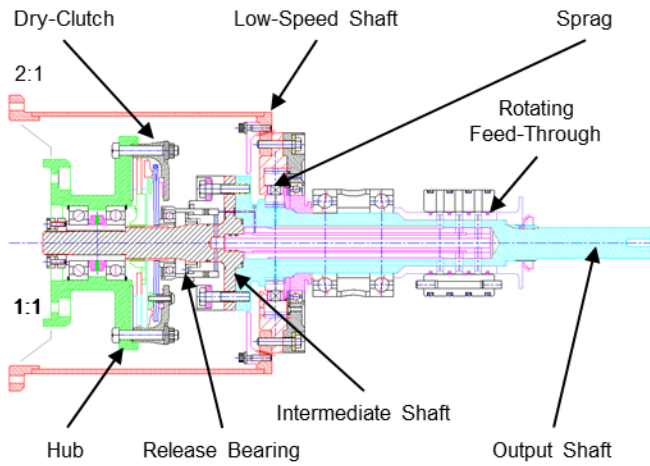
Figure 6. Dry-Clutch Module.
