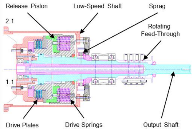
Figure 8. Wet-Clutch Module.
