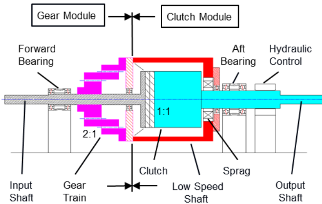
Figure 3. Modules Schematic.
