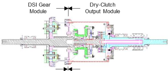
Figure A2. Configuration 2: DSI Planetary / Dry-Clutch
