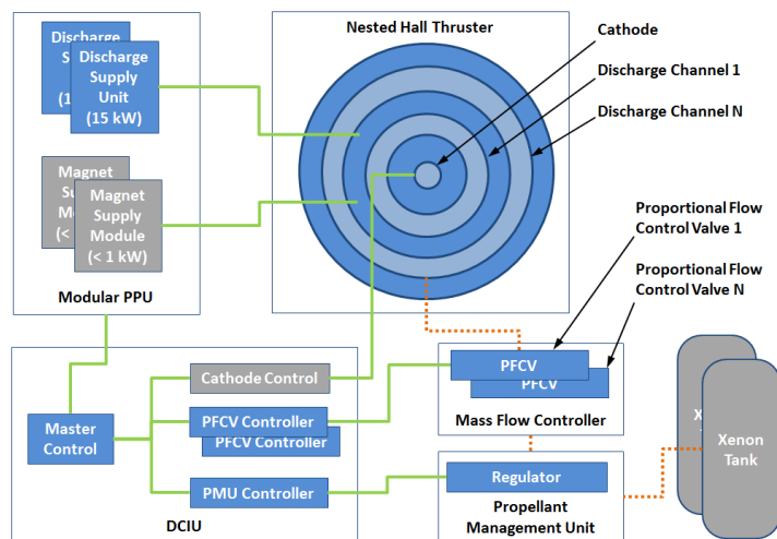
Figure 1. Block diagram of XR-100 system architecture showing modularity chosen to take advantage of NHT wide throttle range. Blue blocks are being developed as part of the NextSTEP program.
