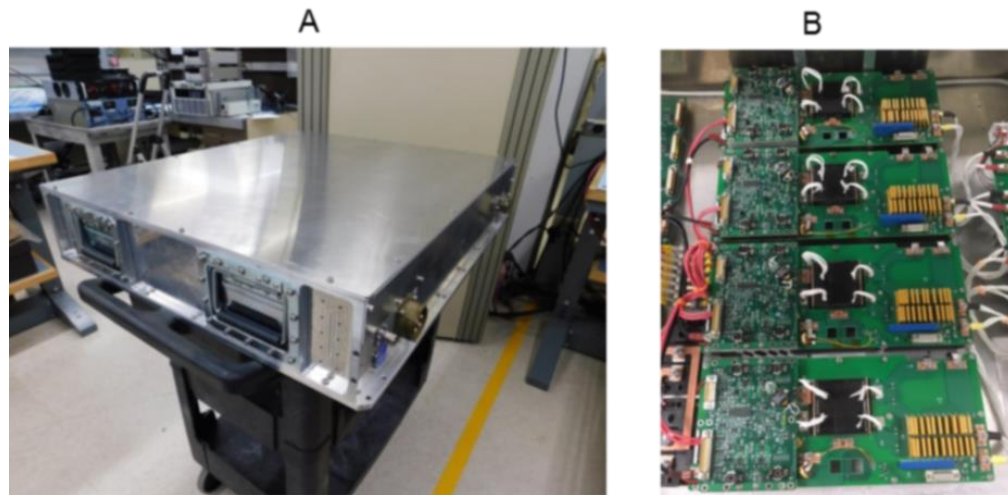
Figure 3. A) Discharge Supply Unit Assembly B) Four Power Modules (PM) inside a Discharge Supply Unit
