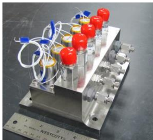
Figure 10. Five-Valve MFC
