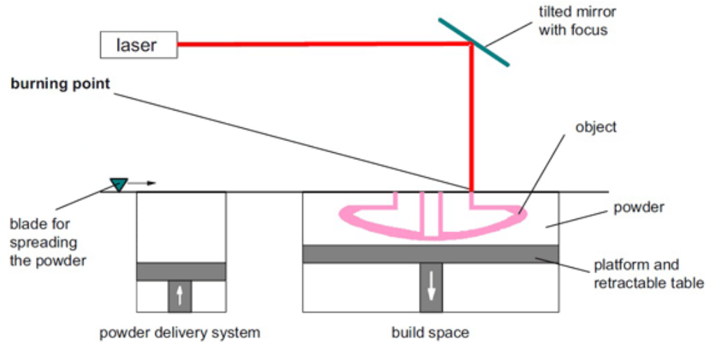
Figure 3. Overview of Selective Laser Melting (SLM) Fabrication Process. [Ref. 10]
