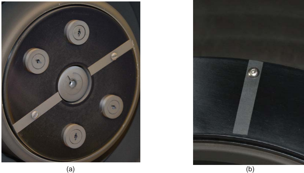
Figure 3.—Masks and bushings installed on the TDU-3 (a) IFPC and keeper and (b) OFPC. The 12 o'clock corresponds to the top of both photos.
