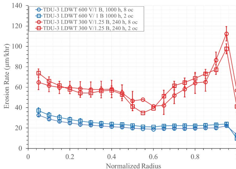
Figure 7.—Comparison of IFPC erosion rates measured near the 8 o'clock (8 oc) and 2 o'clock (2 oc) masks.
