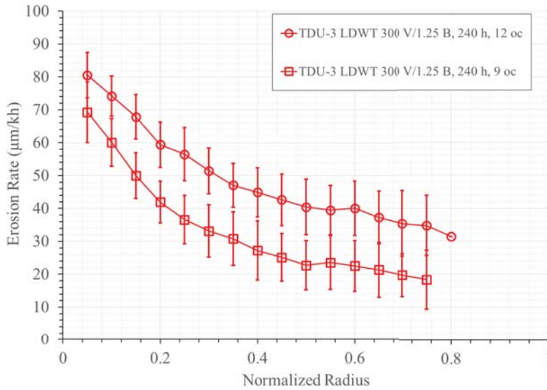
Figure 11.—Comparison of OFPC erosion rates measured near the 12 o'clock (12 oc) and 9 o'clock (9 oc) masks.
