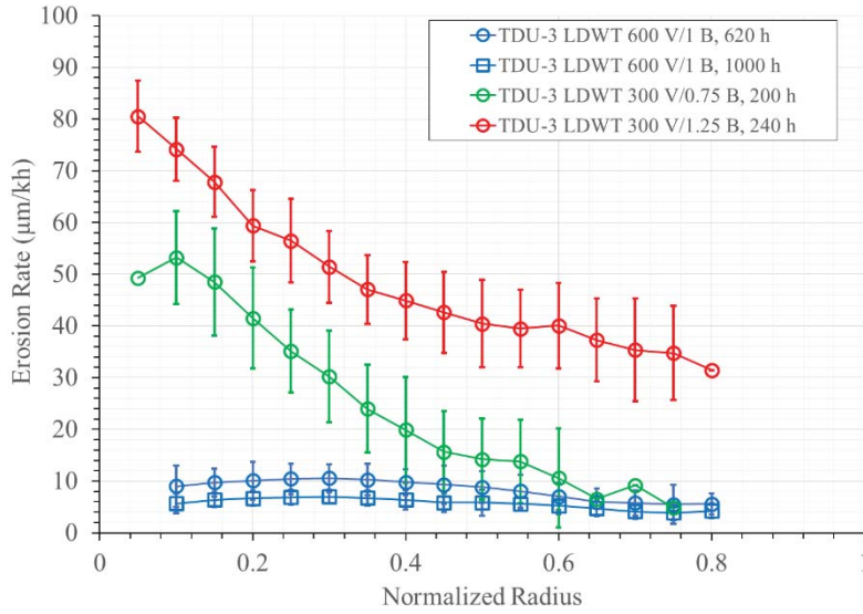
Figure 10.—OFPC erosion rates measured during the TDU-3 LDWT.
