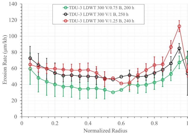
Figure 6.—IFPC erosion rates near the 8 o'clock mask for the three segments performed at 300 V.
