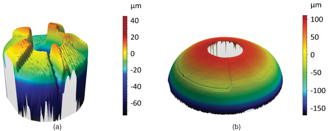
Figure 9.—3D view of the keeper after the (a) SDWT and (b) LDWT (Segment I).
