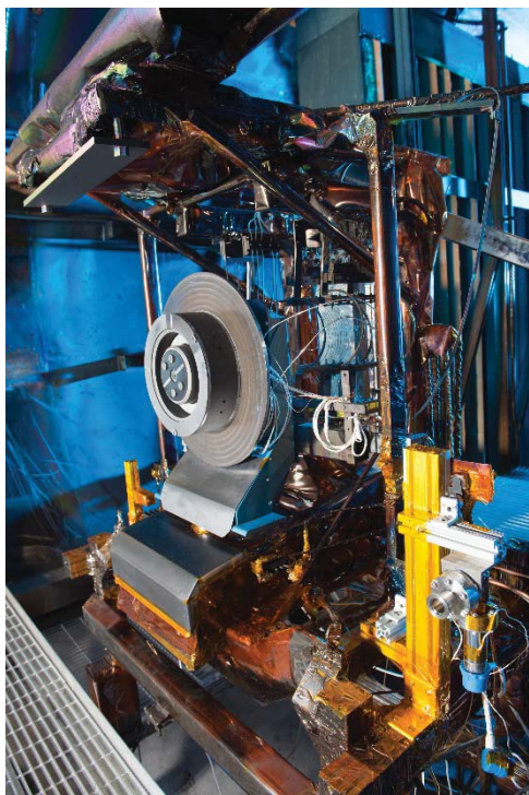
Figure 1.—HERMeS TDU-3 Hall thruster in the configuration used for the LDWT.
