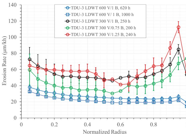
Figure 4.—IFPC erosion rates near the 8 o'clock mask from the TDU-3 LDWT.
