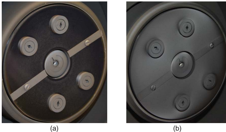
Figure 12.—TDU-3 IFPC (a) before and (b) after completion of a segment of the LDWT.
