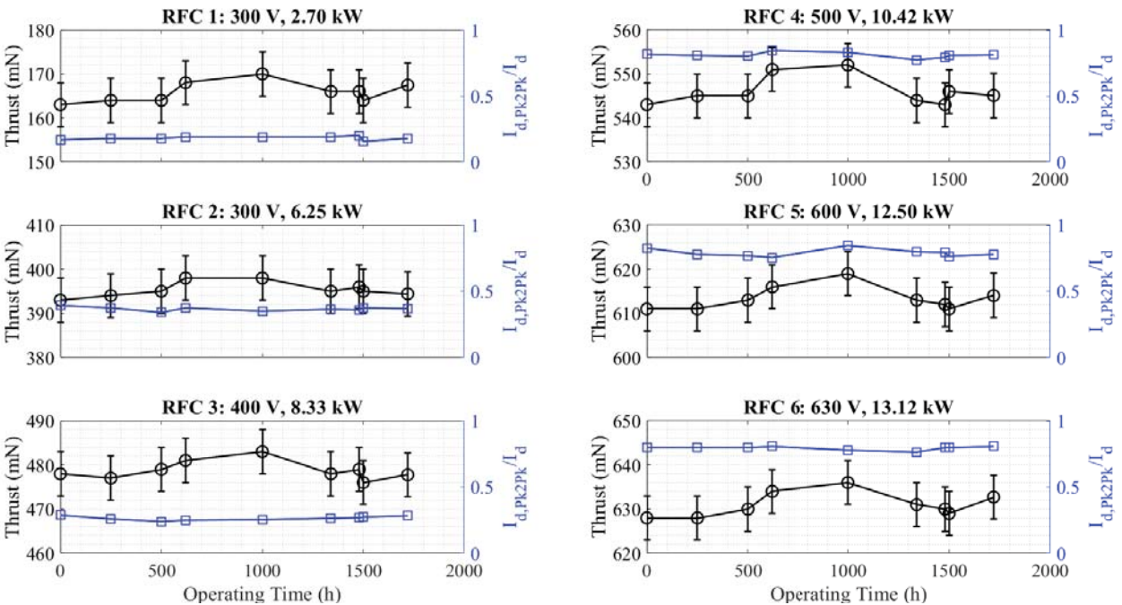
Figure 2.—Performance and stability of TDU-3 during the LDWT at each of the RFCs.
