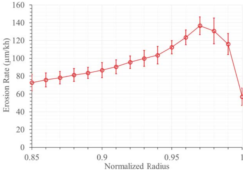
Figure 5.—IFPC erosion rates near a normalized radius of 0.9 for the 300 V/1.25 B condition.
