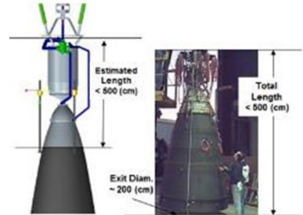
Size comparison: Baseline 25klbf NTP (Left) vs. RL10 (right) (Courtesy Aerojet Rocketdyne)
