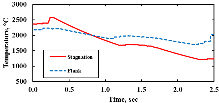
Iron Meteorite (ICCD1) Pyrometer Data: Emissivity 0.3
