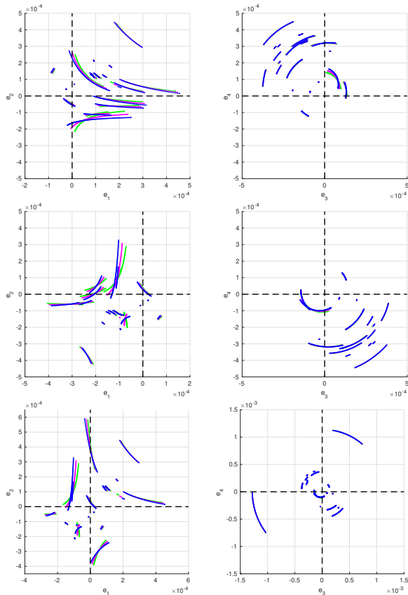
Fig. 14: Projection of Starshade trajectory on the saddle plane \{e_1, e_2\} (left) and center plane \{e_3, e_4\} (right) for cases R01 magenta, R02 green, R03 blue. Top: DRMT trajectory, Middle: DRMA trajectory, Bottom: DRMM trajectory.
