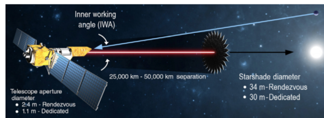
Fig. 1: Representation of the Telescope/Starshade concept.
