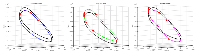
Fig. 11: Trajectory of Different DRM options.
