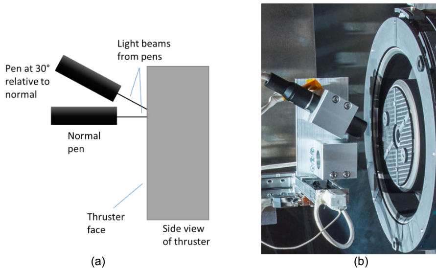
Figure 3.—(a) Diagram of profilometer pen orientation; (b) actual orientation with Hall thruster (only one pen shown).
