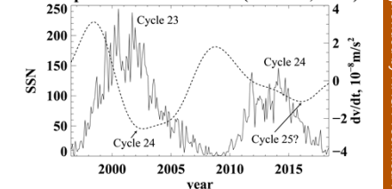
Evolution of the sunspot number (solid curve) and the zonal acceleration (dashed) in the region of initiation of the torsional oscillations, located in the tachocline at 60 degrees latitude.
