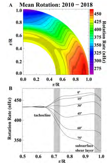
(A) The mean solar rotation rate profile obtained from the SDO/HMI data. Dashed line indicates the tachocline and the subsurface shear layer. (B) The mean rotation rate as a function of radius at different latitudes. The gray intervals indicate the tachocline and the subsurface shear layer.
