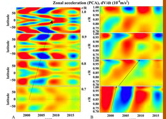
(A) Time-latitude diagrams of the zonal acceleration at four different depths of the convection zone (the corresponding radii: r/R=0.7, 0.8, 0.9 , and 1.0 ), obtained after applying the Principal Component Analysis. Inclined line with arrows marks the end of Solar Cycle 23 at 0.7R and 1.0R . (B) Time-radius diagrams at four different latitudes: 5^\circ, 15^\circ, 30^\circ , and 45^\circ . Inclined lines with arrows the direction of migration of the low and latitude torsional oscillation branches corresponding to Cycle 24.
