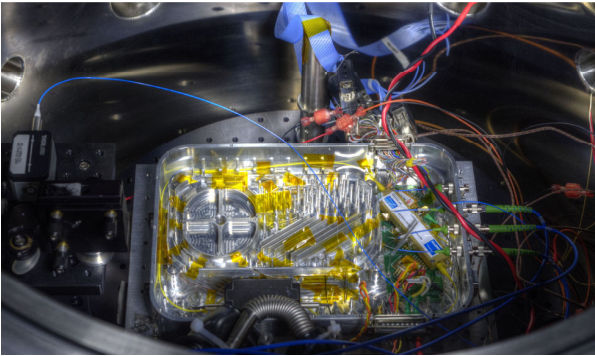
Figure 6. Photo of the baseline fiber amplifier built at NASA/GSFC. It is set in a thermal vacuum chamber for environmental testing.
