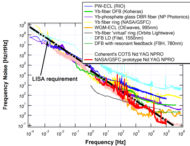
Figure 4. Free-running frequency noise spectrum of various single-frequency lasers near 1um.
