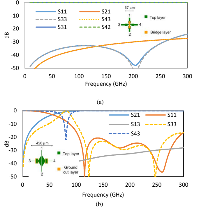
Fig. 4. Simulated S-parameter response using HFSS of (a) vacuum bridge compared to (b) via-less crossover as a function of frequency. The via-less crossover signal crosses on the ground plane side from port 3 to 4.
