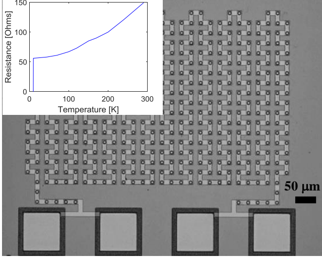
Fig. 3. Four wire crossover chain consisting of a series array of 264 niobium crossovers with inset showing superconducting transition of series array structure.
