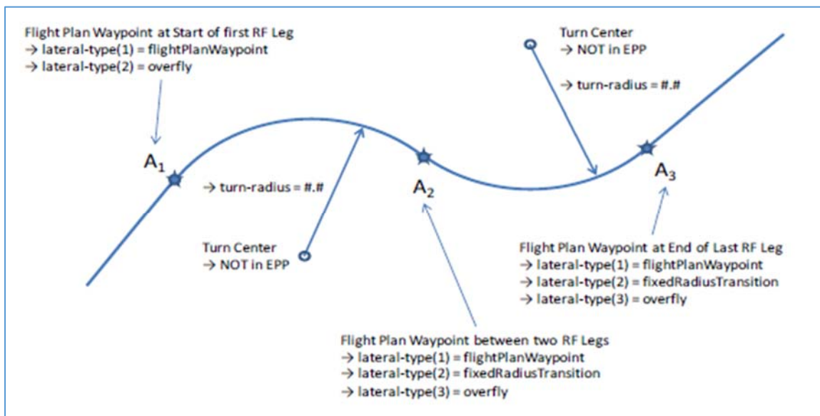
Figure 12. RF Legs 23
