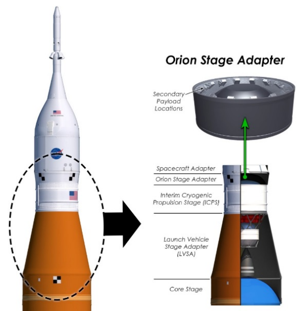
Fig. 7. At the top of the Block 1 configuration, the Orion Stage Adapter has capacity for up to 19 smallsats; the SLS Program provides an integrated deployment system for the payloads.
