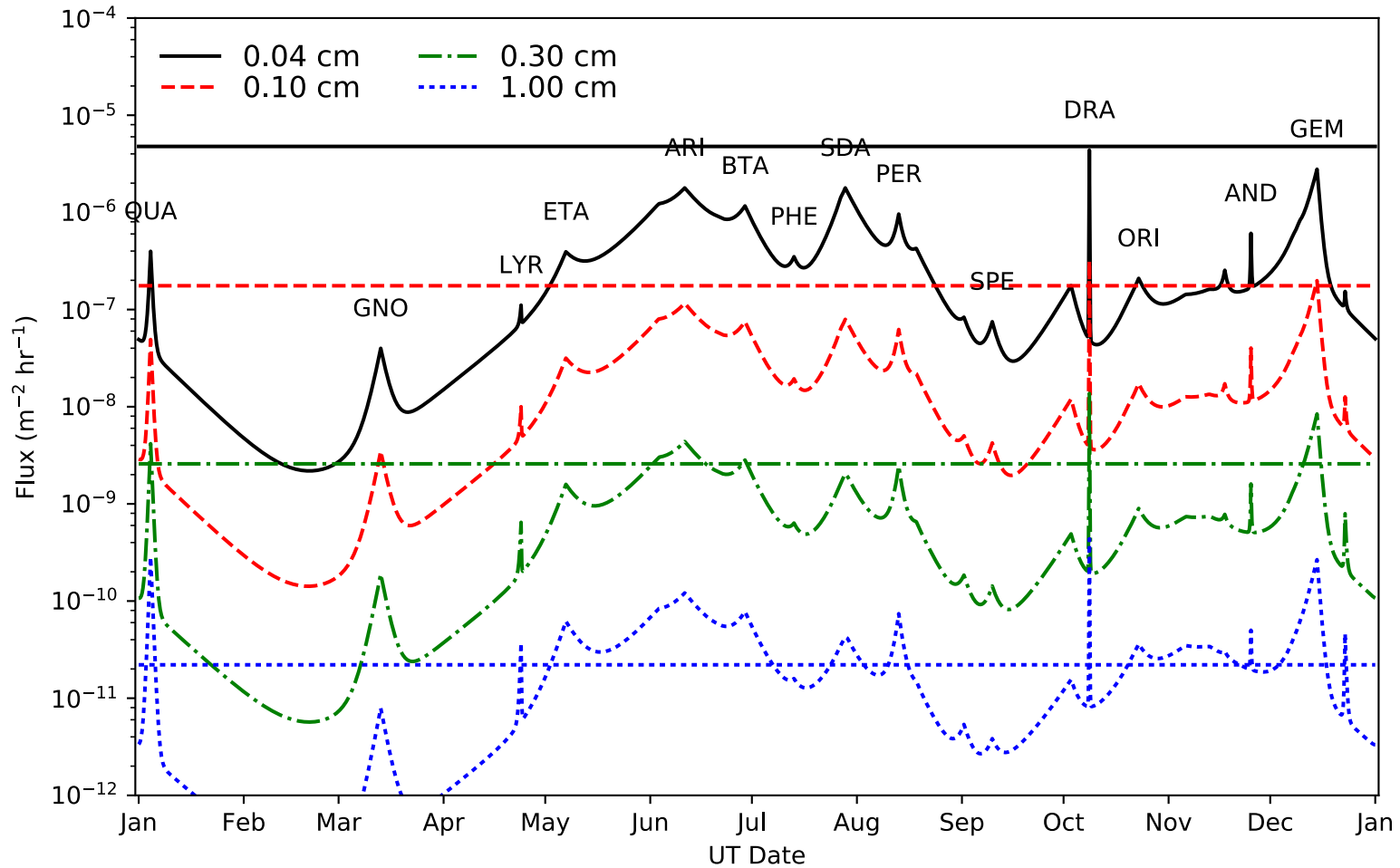
Figure 2: Meteor shower flux (variable lines) and sporadic meteoroid flux (horizontal lines) over the course of 2019. Fluxes have been weighted to a constant limiting kinetic energy. Fluxes are quoted for four particle kinetic energies; these kinetic energies correspond to particles with diameters of 0.04 cm, 0.1 cm, 0.3 cm, and 1 cm, assuming a density of 1 g/cc and a speed of 20 km/s. Some showers, such as the Perseids (PER) and Quadrantids (QUA), are more heavily weighted toward large particles and thus play a more significant role for 1-cm-equivalent particles than for 0.04-cm-equivalent particles.
