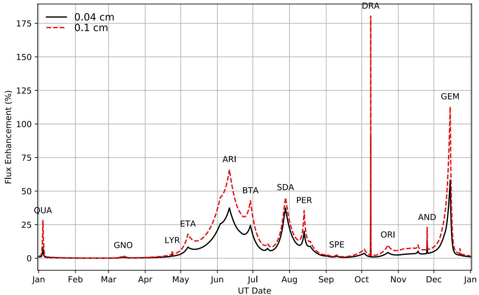
Figure 3: Meteor shower flux enhancement relative to the sporadic meteoroid flux over the course of 2019. These factors can be used in conjunction with a meteoroid model such as the Meteoroid Engineering Model (MEM) to compute the flux at a particular point in the year on a plate facing the unobscured shower radiant.
