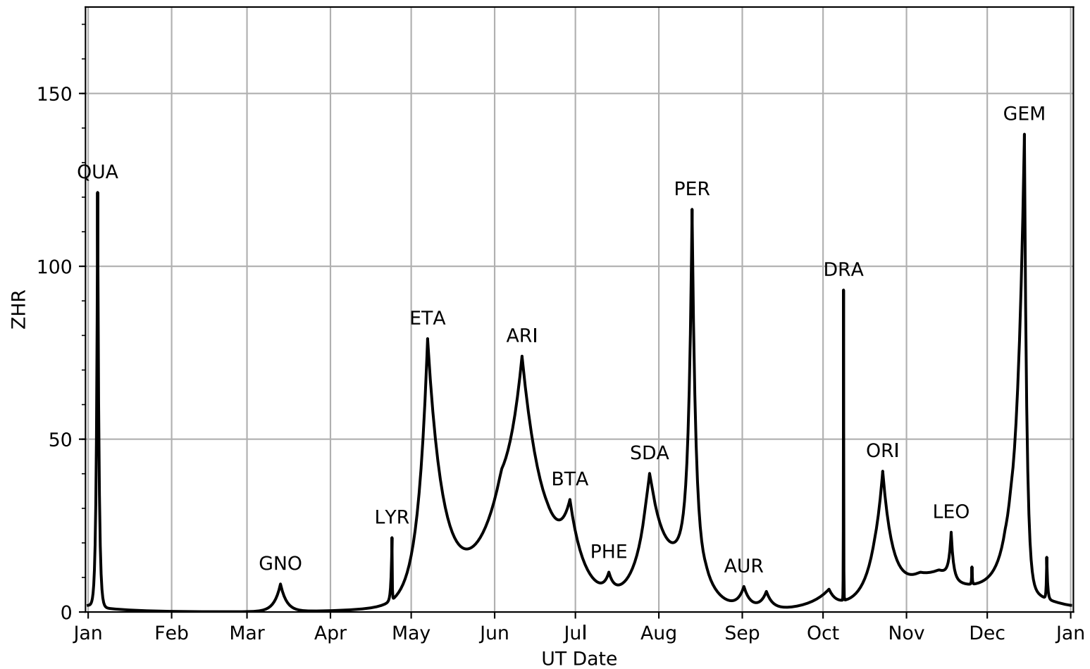
Figure 1: Meteor shower visual rates (zenithal hourly rate, or ZHR) over the course of 2019. Note how showers overlap; a large, broad shower such as the Daytime Arietids (ARI) can boost the cumulative shower ZHR and flux at the peak of an adjacent shower (reflected in column 4 of Table 2).
