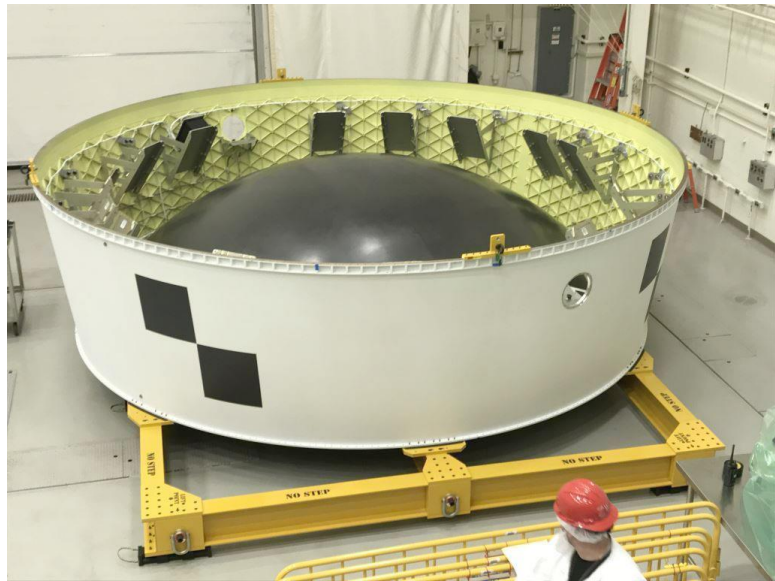
Figure 12. The Orion Stage Adapter (OSA), prior to shipping to Kennedy Space Center (KSC), showing the mounting brackets for the secondary payload dispensers and avionics unit
