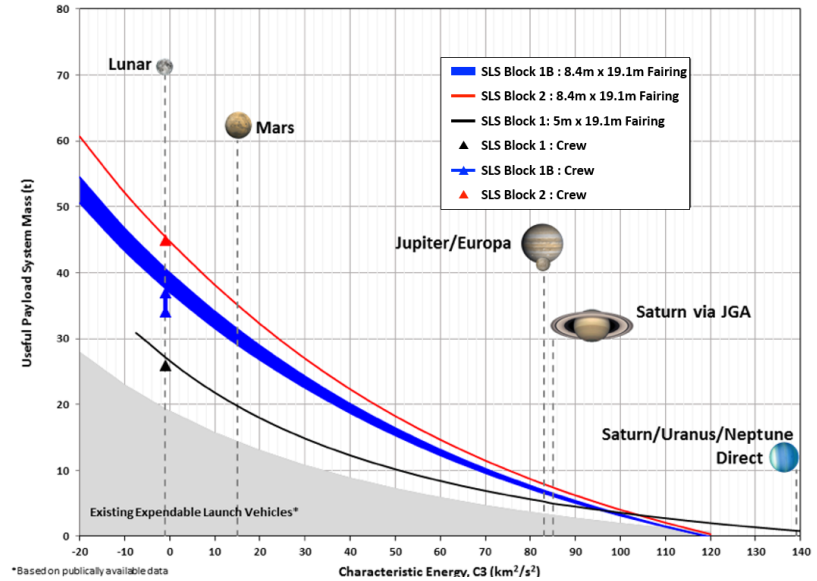
Figure 6. SLS vehicles can deliver a range of useful payload mass, shown here as a C3 curve
