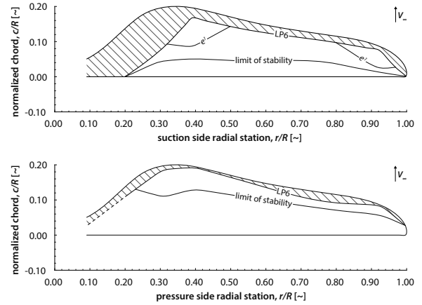
Figure 18. Mars Helicopter upper rotor, approximated compressible two-dimensional boundary layer state in hover for Mars Condition 2 at 2,800 RPM
