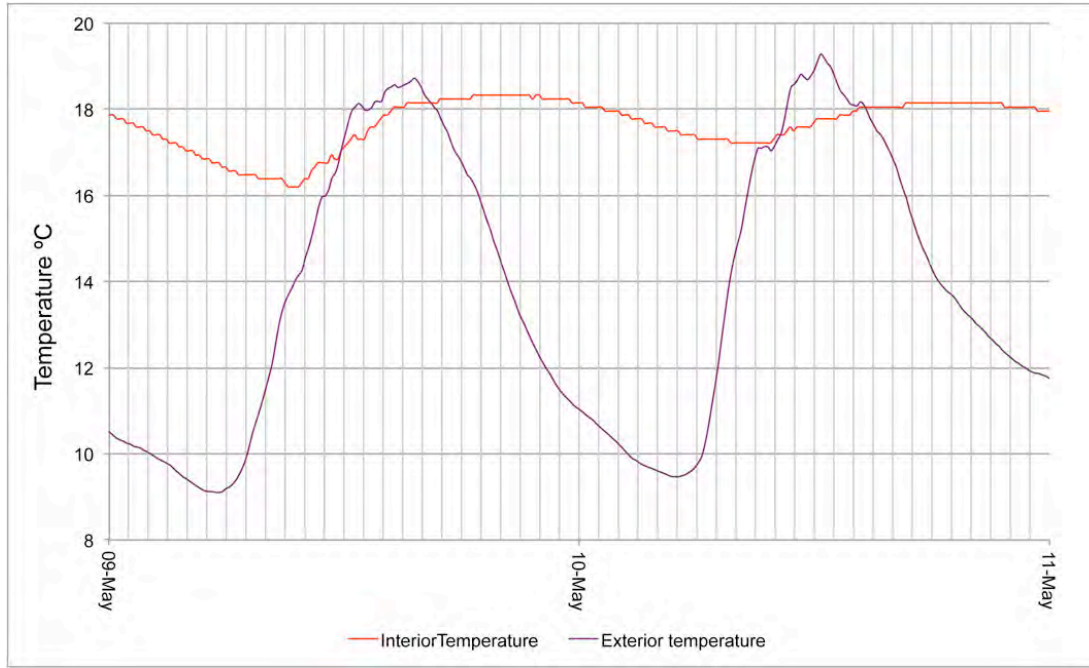
Figure 12: Thermal phase shift through the HemPod walls
