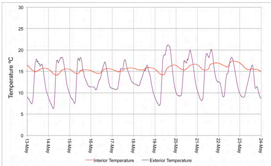
Figure 4: Internal and external temperature in the HemPod
