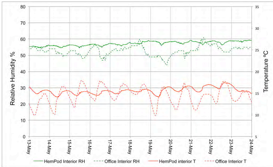
Figure 11: Temperature and Relative Humidity inside the office (dotted lines) and the HemPod (solid lines)
