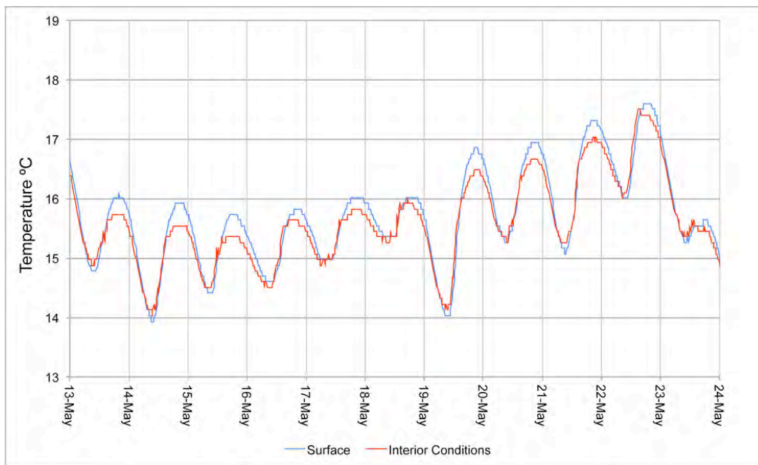
Figure 7: Comparison between internal environmental temperature and wall surface temperature (HemPod)
