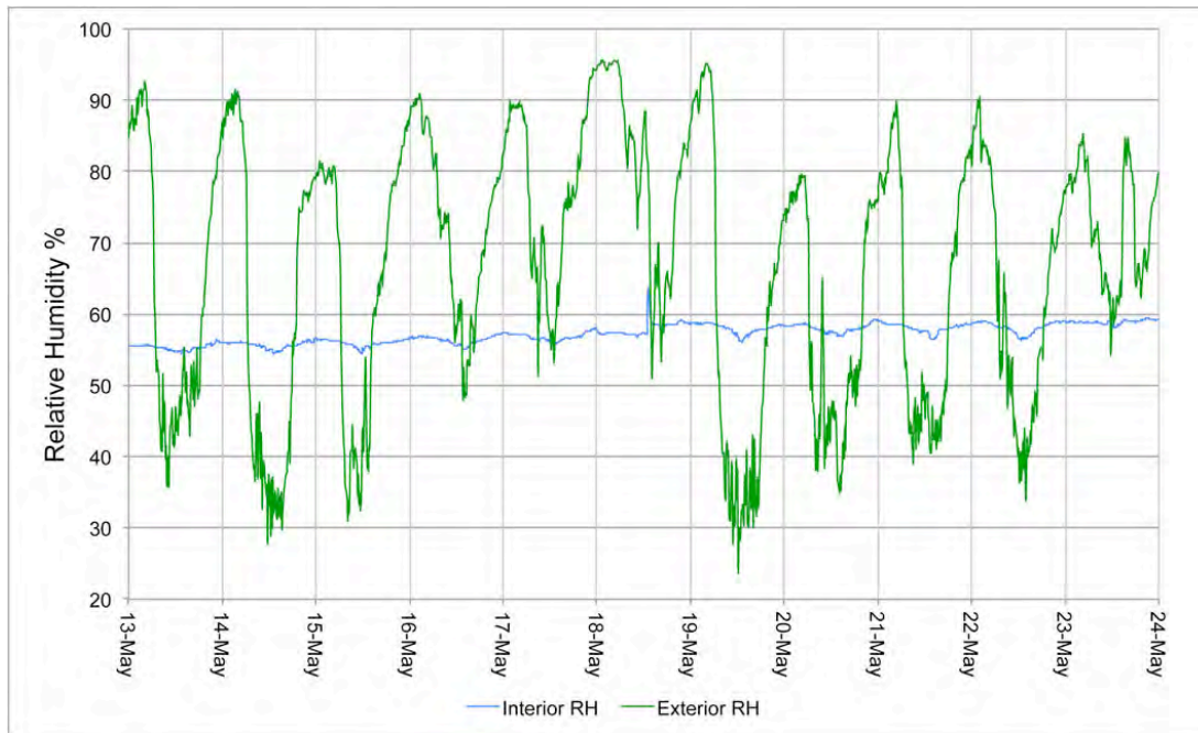
Figure 9: Internal and external relative humidity for the HemPod
