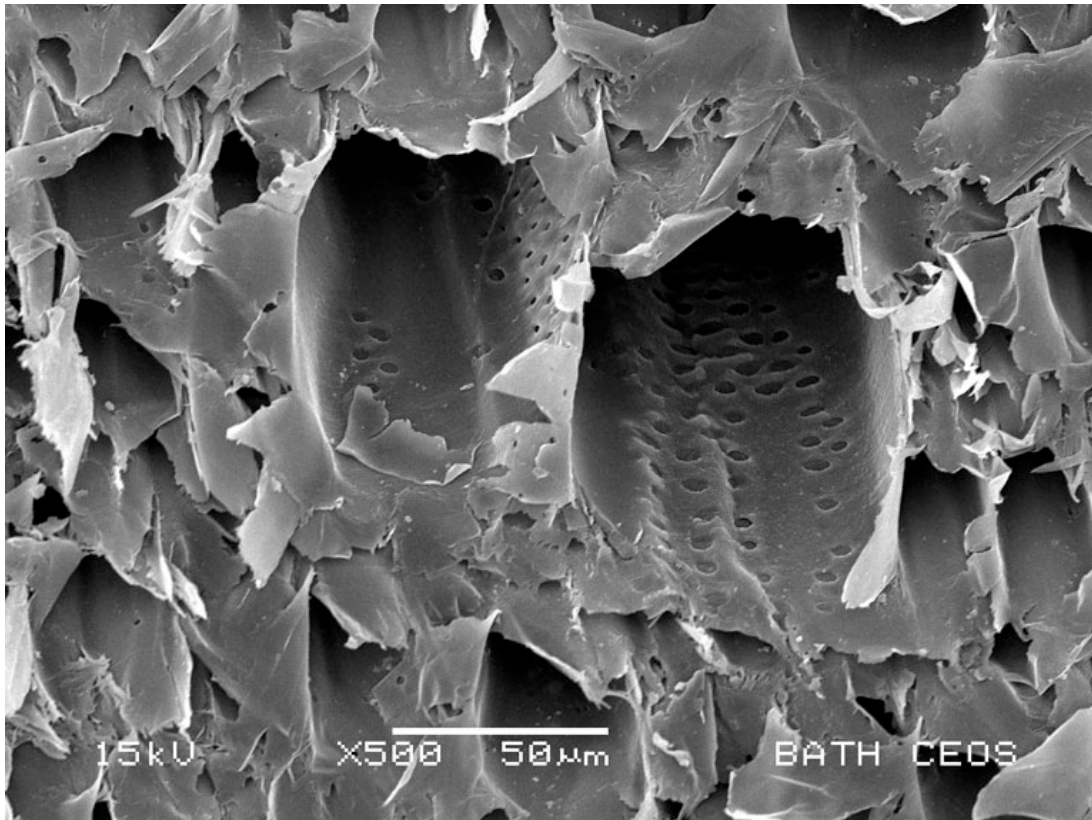
Figure 13: Interlinked pore structure of hemp shiv (Photomicrograph x 500)
