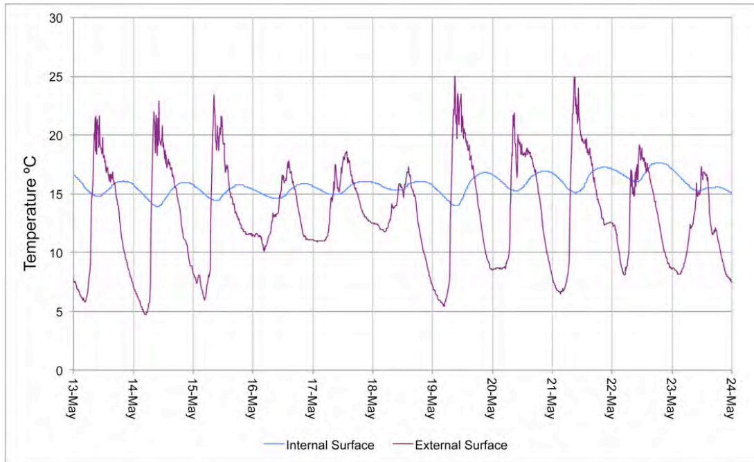
Figure 6: Comparison of the internal and external surface temperatures (HemPod)
