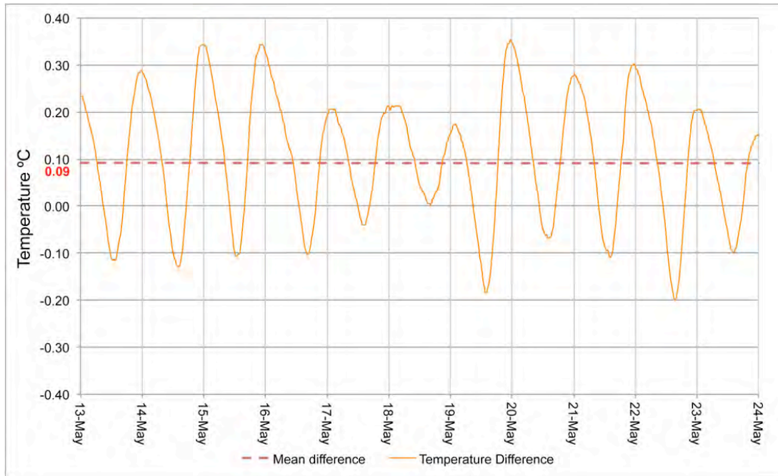
Figure 8: Temperature difference between surface and air temperature (HemPod)
