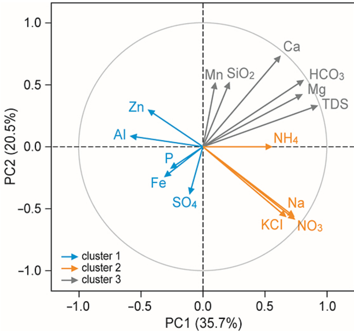
Figure 5. PCA plot of the macro-ionic content of the water samples. Arrow lengths indicate the variable loadings (ion composition) along the PCA axes, where the maximum of each loading is 1. The clusters indicate the proportionality relation between the variables and the PCA axes.
