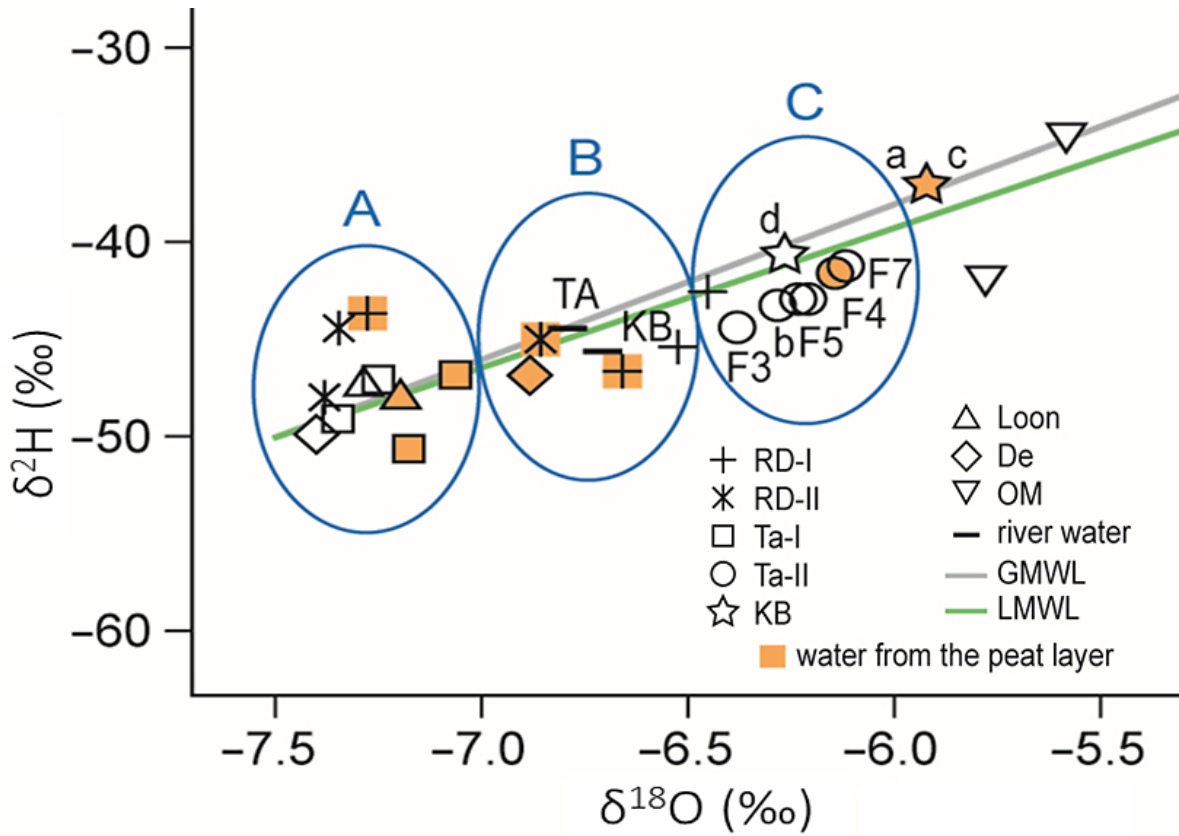
Figure 4. Stable isotopic compositions were plotted with GMWL and LMWL. Water samples collected from the peat layers are indicated with yellow filling.
