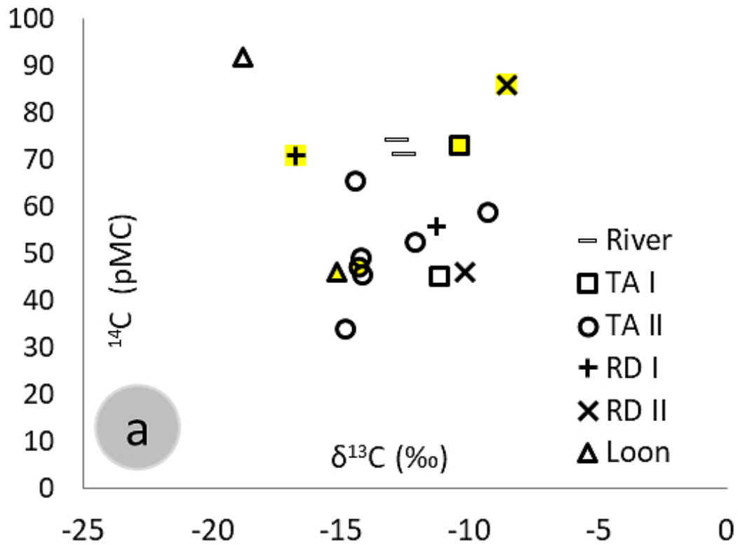
Figure 3. Relationships of the ^{14}\text{C} (pMC) content in the water samples with (a) \delta^{13}\text{C} (‰), and (b) the reciprocal of \text{HCO}_3 (mg/l).
