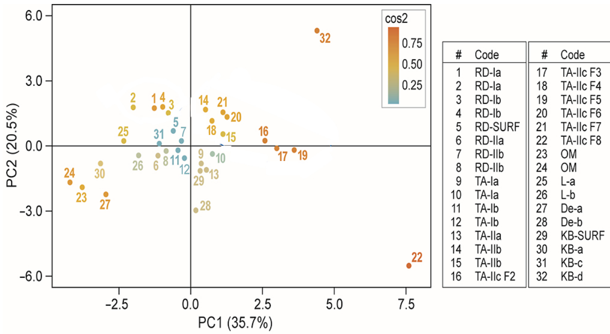
Figure 6. PCA plot of the sampling sites indicating correlations of the water samples to the first two PCA axes. The statistic cos2 indicates the quality of representation (contribution) of the samples by these two PCs. Site codes are: RD-I= Rolderdiep-I, RD-II = Rolderdiep-II, TA-I = Taarlo-I, TA-II = Taarlo-II, OM = Oudemolen, L = Loon, De = Deurze, KB = Kappersbult.
