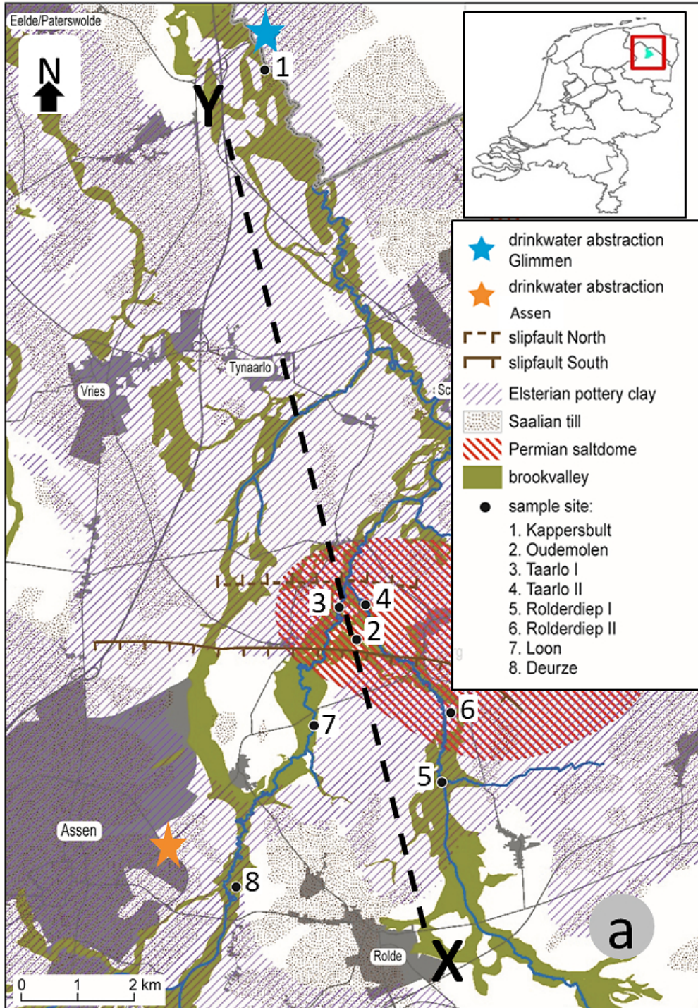
Figure 2 . Groundwater sampling sites and geological features that control the flow patterns in the groundwater (a), simulation model results show the effect of the double diffusion convection along the X-Y transect in (a), which affects groundwater reaching the surface (b).
